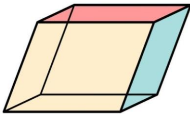
Fig. 3: Parallelepiped
